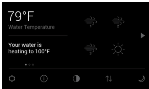
Home Screen
