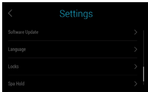
SettingsMenu
